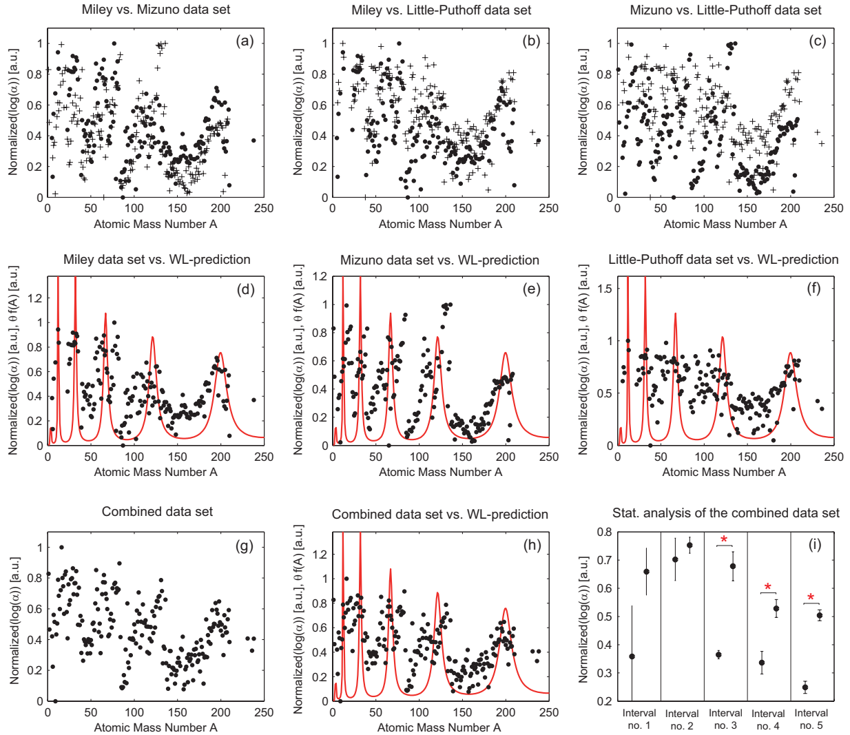
Figure 3. (a)–(c) Comparison of the each data set with each other. \alpha is the scaling of the original data sets (isotopic abundance, ...). (a): Miley ( \bullet ) vs. Mizuno data set (+). (b): Miley ( \bullet ) vs. Little-Puthoff data set (+), (c): Mizuno ( \bullet ) vs. Little-Puthoff data set (+). (d)–(f): Comparison of the each data set with the WL-prediction. Values obtained for the scaling parameter \theta : case (d), \theta = 0.751 ; case (e), \theta = 0.655 ; case (f), \theta = 0.3703 . (g)–(h): Comparison of the sum of all data sets with the WL-prediction. (g) Combined data set. (h) Combined data set vs. WL-prediction. (i) Result of the interval analysis. * Indicates statistically significantly ( p < 0.05 ) differences.
